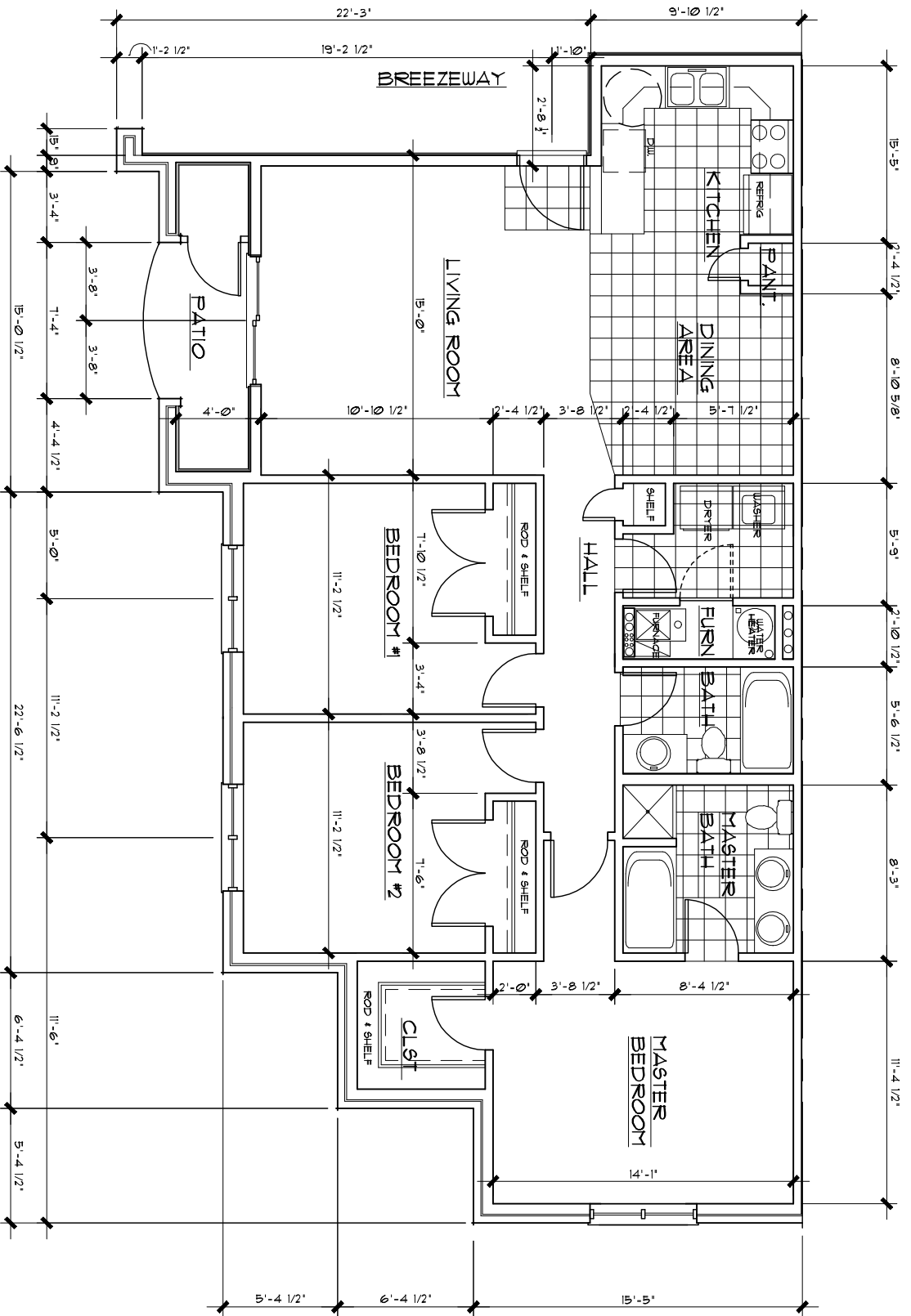
SECOND/THIRD FLOOR PLAN - THREE BEDROOM UNIT 1,174 SQUARE FEET
